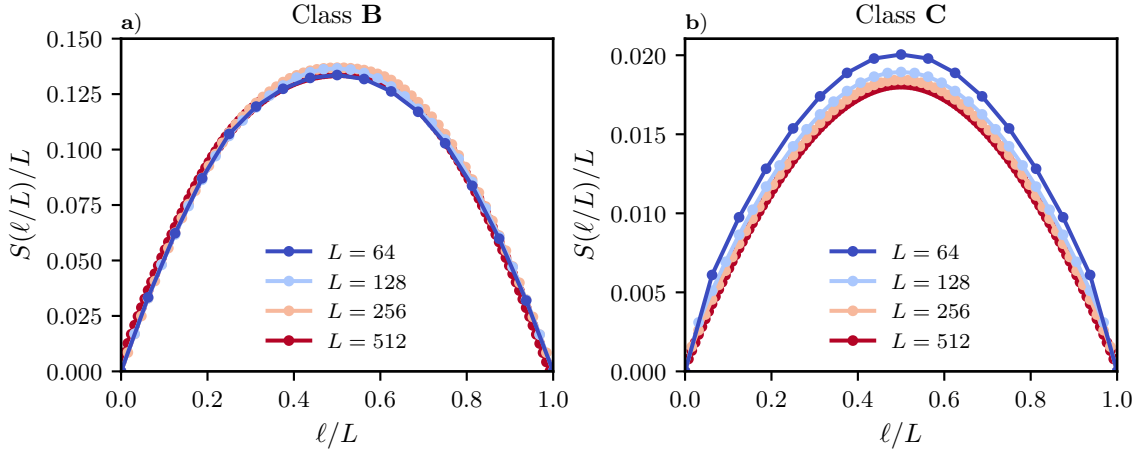
Figure 15: Steady-state entanglement entropy as a function of the subsystem fraction \ell/L in the volume-law phase for Class B (a) and Class C (b). Other parameters: \nu = 1/4 , \nu_0 = 1/4 , \gamma = 0.5J , and h = J .
