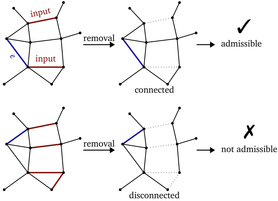
Figure 3: Illustration of the admissibility concept. Top: The removal of the input edges results in a connected graph, satisfying the criterion for admissibility. Bottom: The resulting graph is disconnected thus the input set is not admissible.
