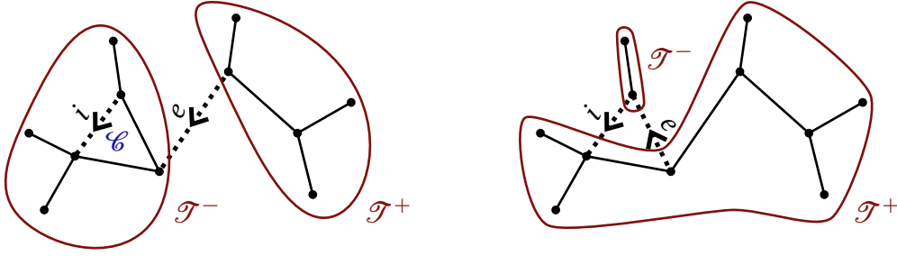
Figure 5: Resulting graph after removal of \mathcal{I} and e Left: e and i do not belong to the same cycle \mathcal{C} , notice that i is fully contained by \mathcal{T}^- . Right: Since e and i belong to the same cycle, i is in between both trees \mathcal{T}^\pm .
