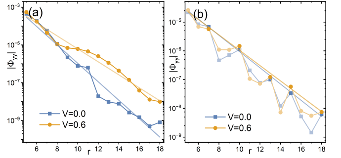
FIG. 4. SC correlation functions \Phi_{yy}(r) for (a) t' = 0.0 in the charge stripe phase and (b) t' = -0.4 in the holon Wigner Crystal phase. Solid lines denote exponential fits \Phi(r) \propto e^{-r/\xi_{sc}} .
