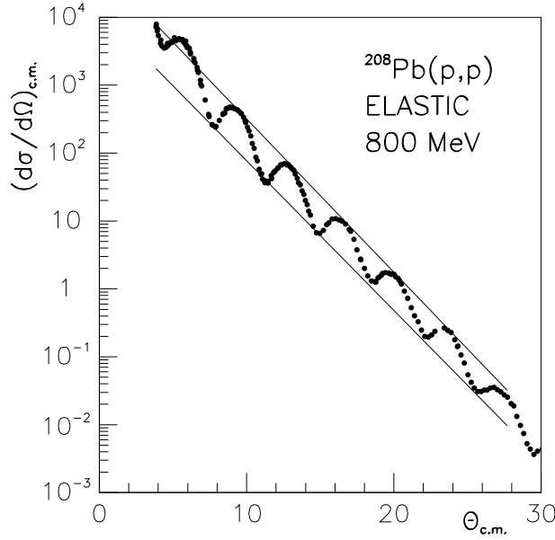
Figure 3: Differential cross section for elastic proton-lead scattering at 800 MeV [5].
