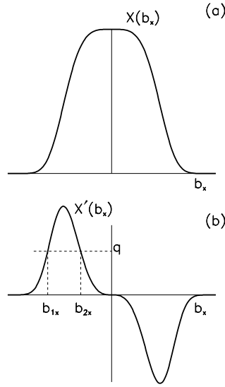
Figure 4: (a) A simple, real, phase shift function X(b_x) and (b) its derivative X'(b_x) . For values of q that are not too large, there are paired trajectories at b_{1x} and b_{2x} . The stationary points are located at negative values of b_x , since a positive phase shift function corresponds to attraction.
