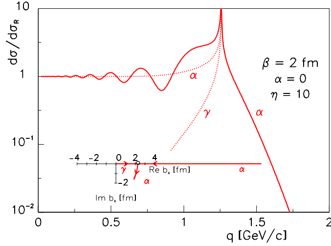
Figure 5: Scattering from the charge distribution (17), normalized to the Rutherford cross section. The dotted curves show the individual contributions from the two stationary points. The inset shows how the stationary points move with increasing momentum transfer.
